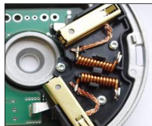
Stranded Wire to Terminal
